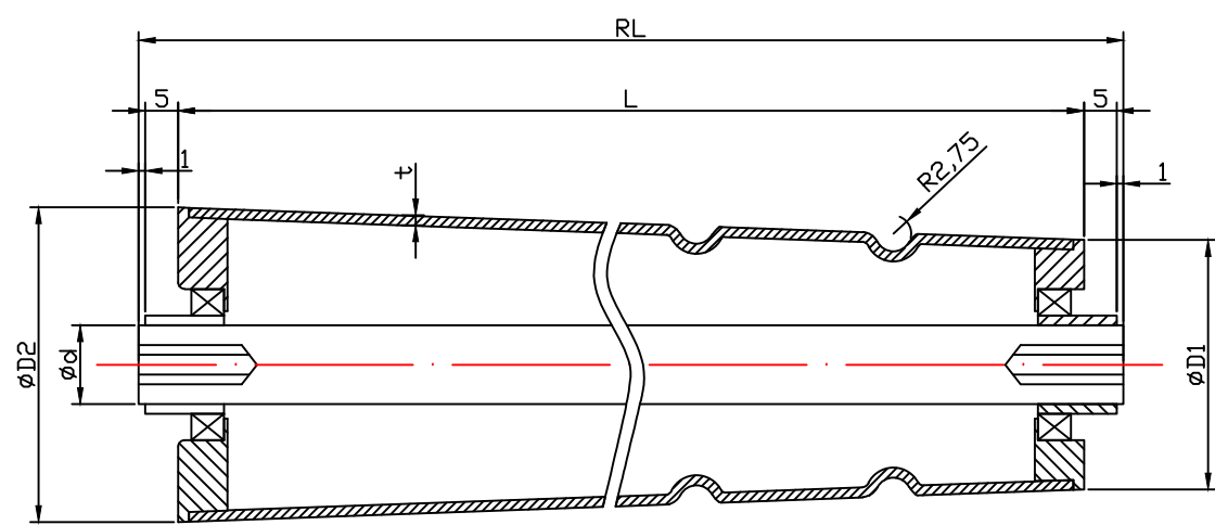
Tapered Double Groove Roller
